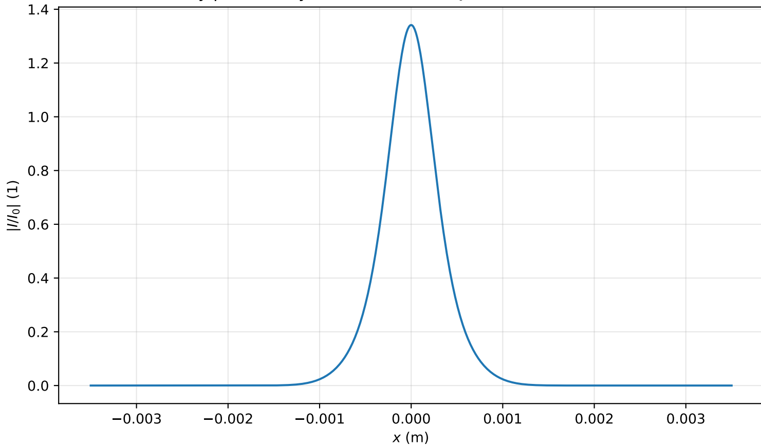
Intensity profile I(x, y = 0, z = 0.876m)/I_0 , P_{in}=0.9P_{cr} , artificial time
